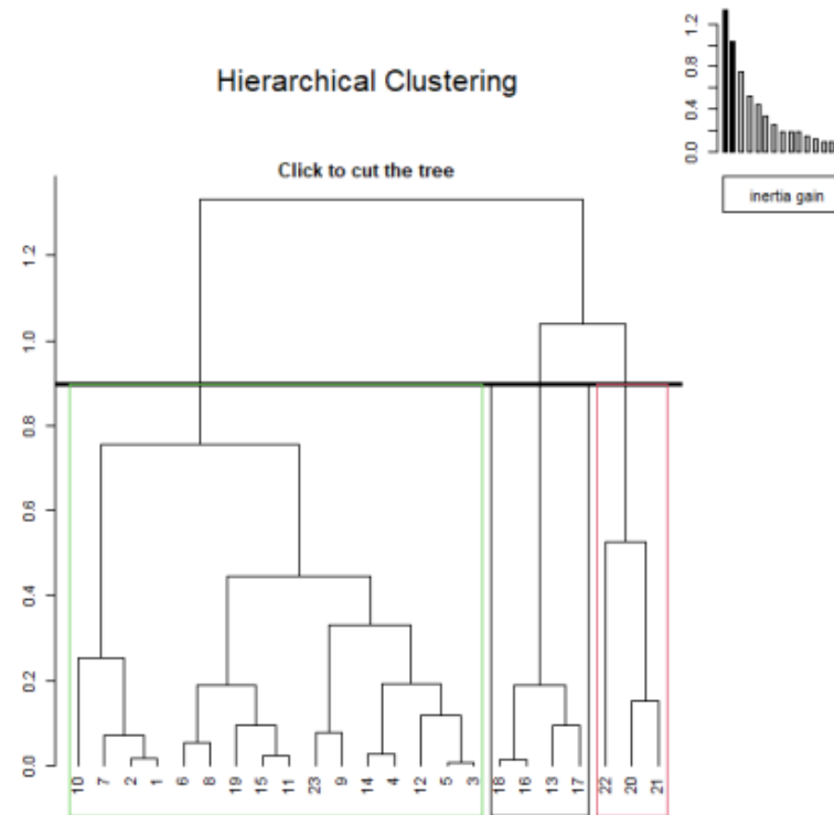
Dendrogramme
