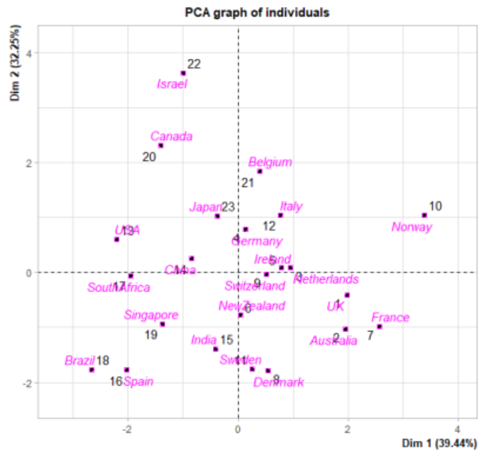
Factor Map
